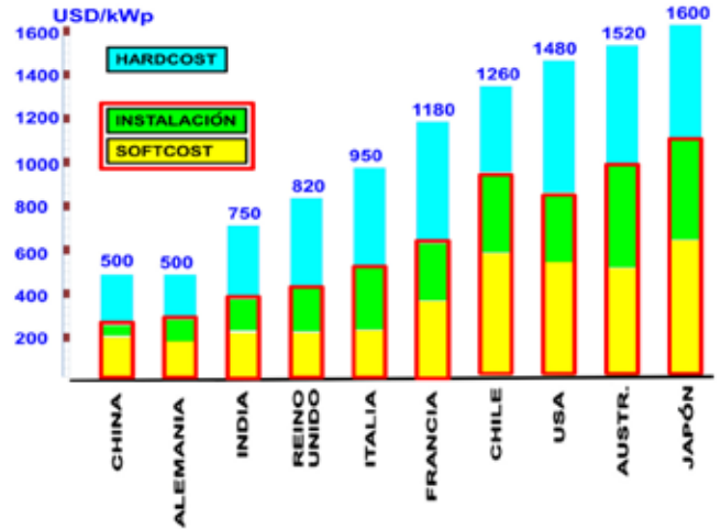
Fig. 7. Costos FV utility.
